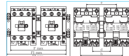
图8 CJX2s(K)-40N~95N
