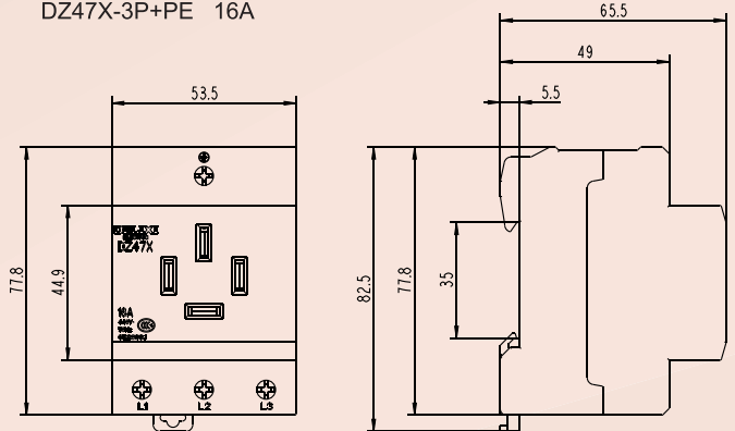
DZ47X-3P+PE 16A
